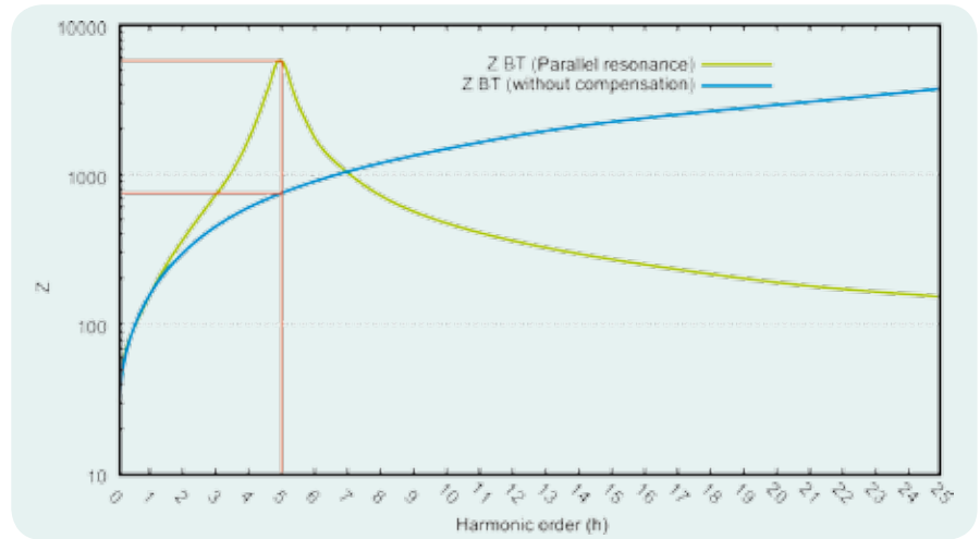
Resonance curve
